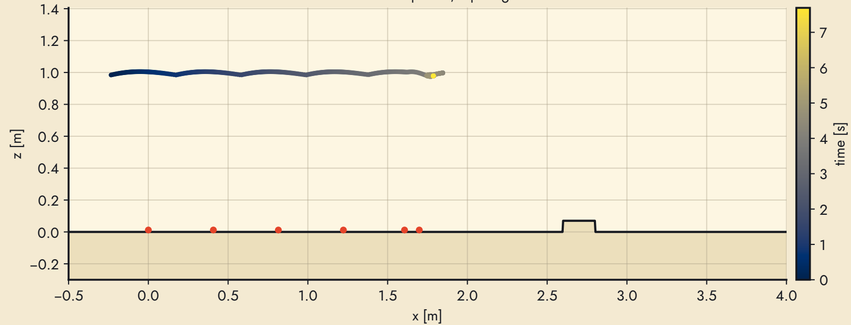
Crate #2: 7 x 20 cm: side profile, hip height and footholds
