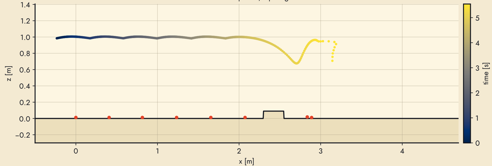
Crate #3: 9 x 25 cm: side profile, hip height and footholds
