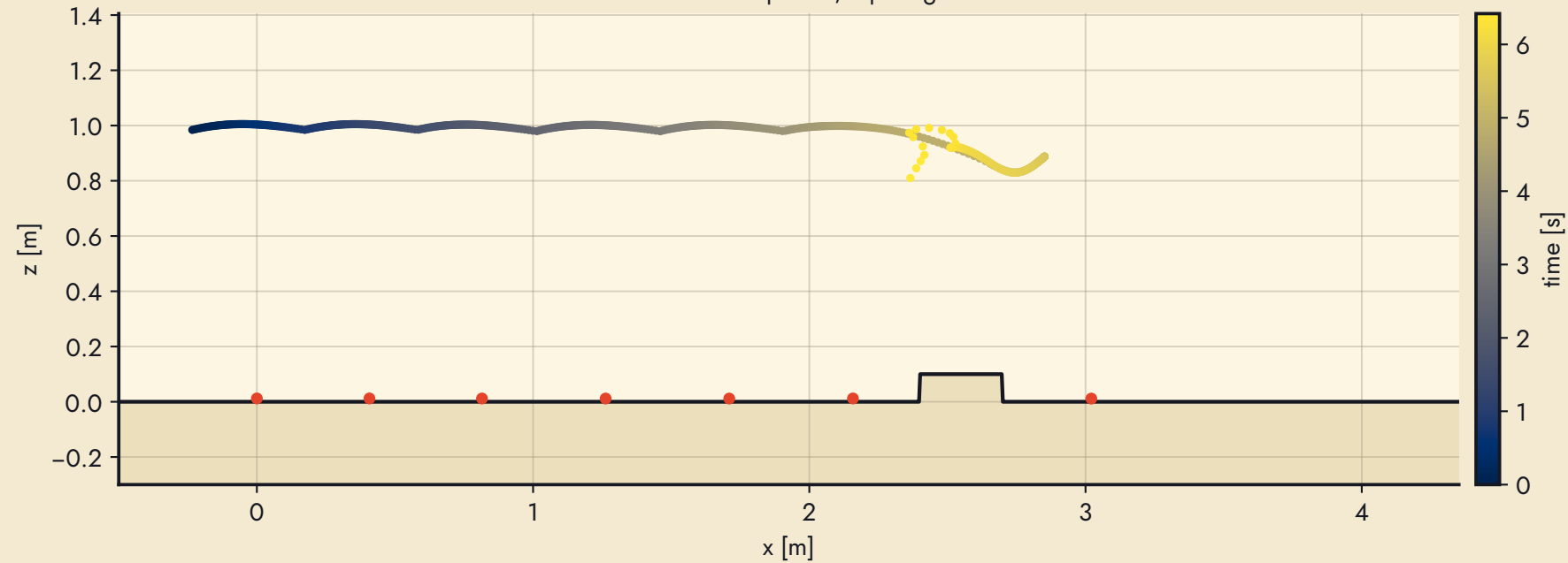
Crate #5: 10 x 30 cm: side profile, hip height and footholds
