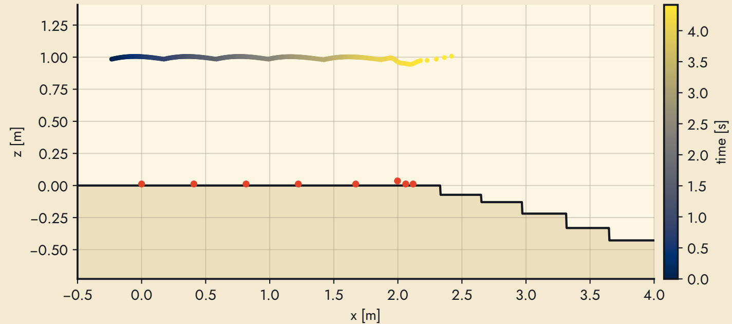
Stairs down #10: side profile, hip height and footholds
