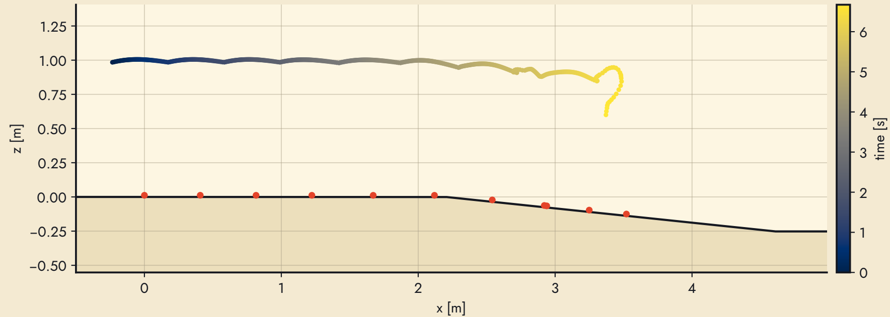
ramps: side profile, hip height and footholds
