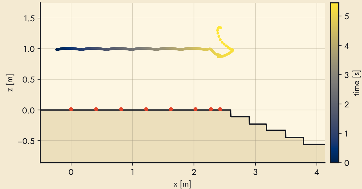
stairs_down: side profile, hip height and footholds
