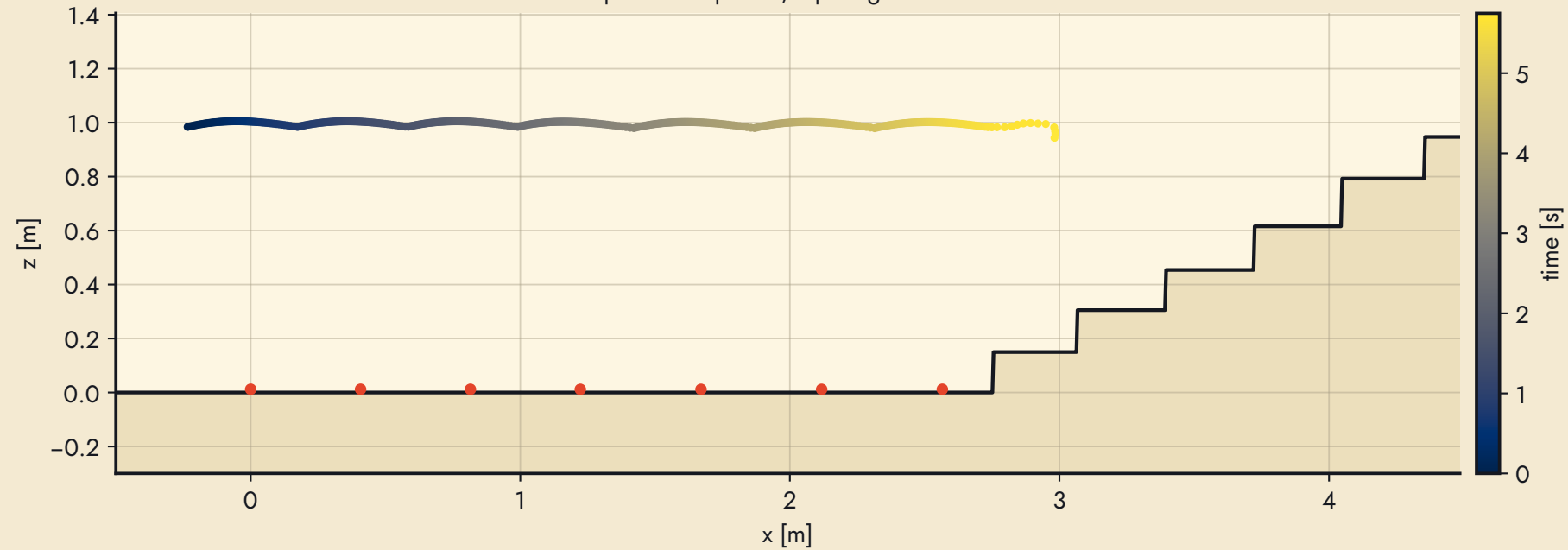
Stairs up #1: side profile, hip height and footholds
