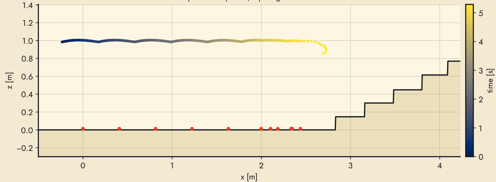
Stairs up #2: side profile, hip height and footholds
