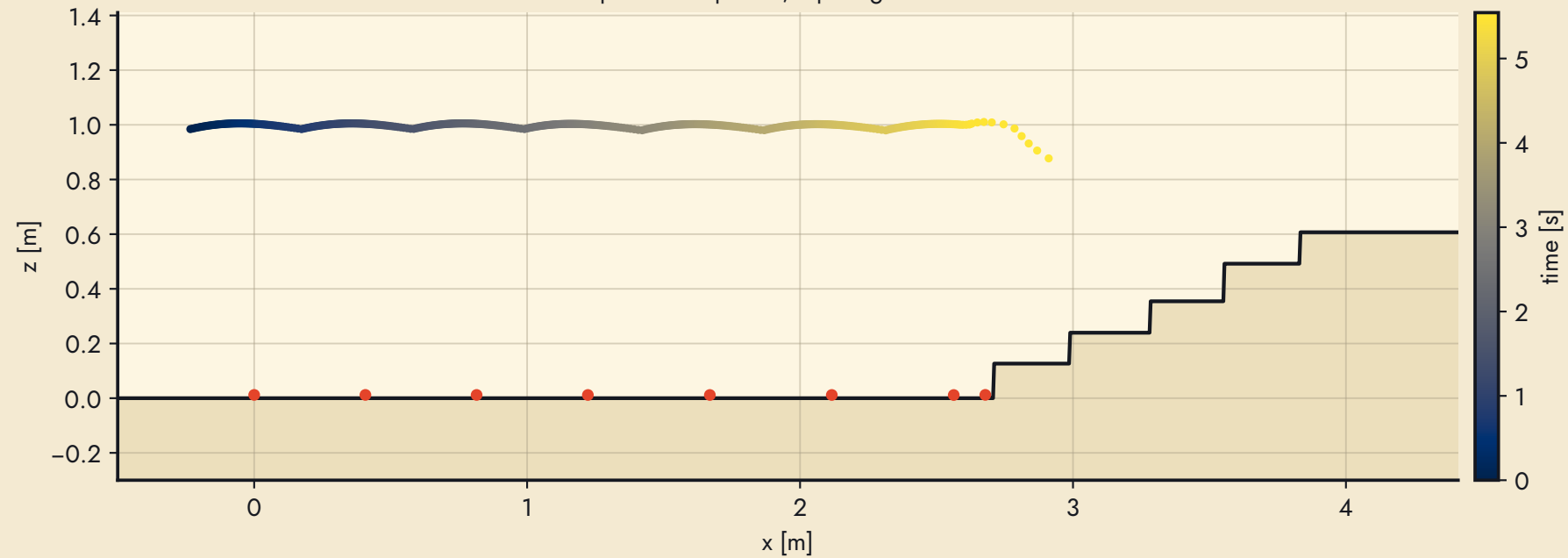
Stairs up #3: side profile, hip height and footholds
