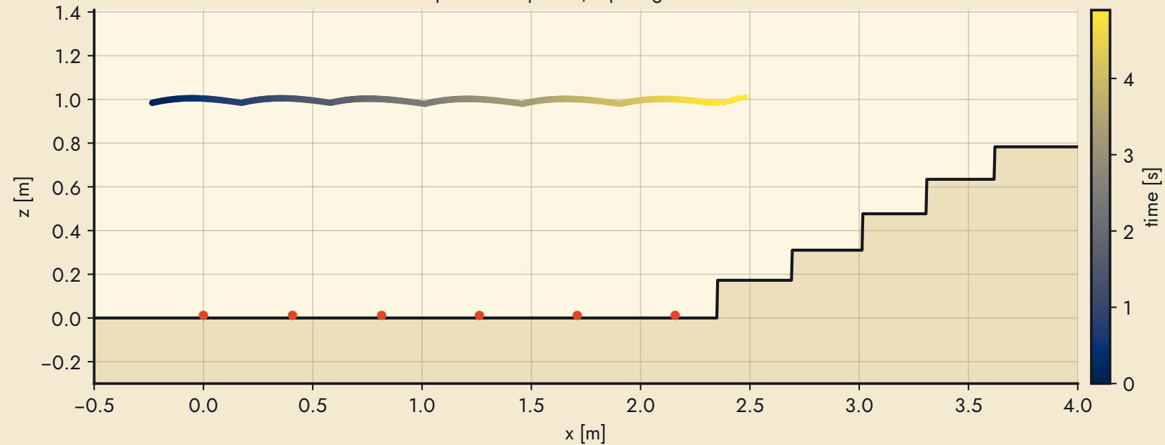
Stairs up #4: side profile, hip height and footholds
