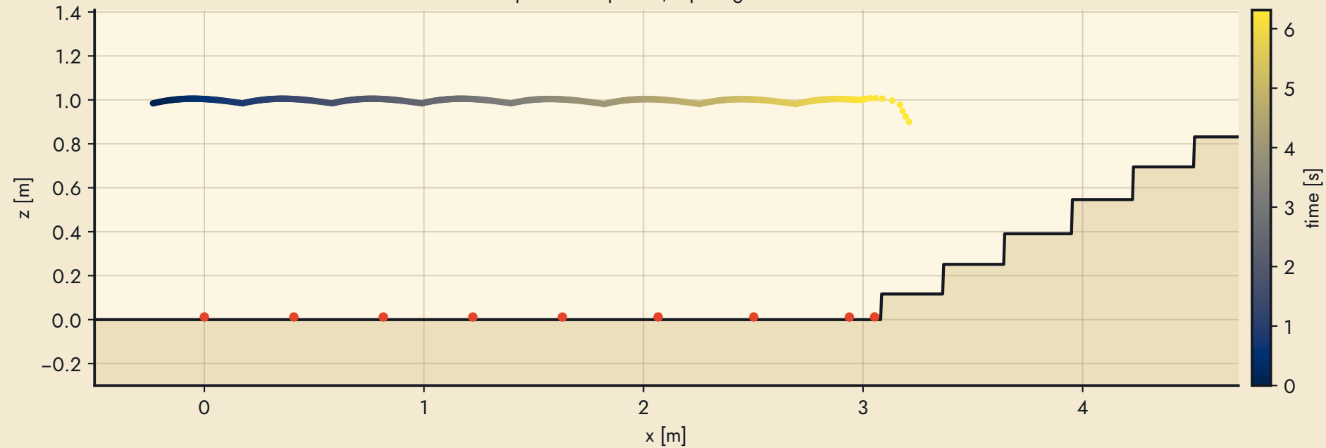
Stairs up #6: side profile, hip height and footholds
