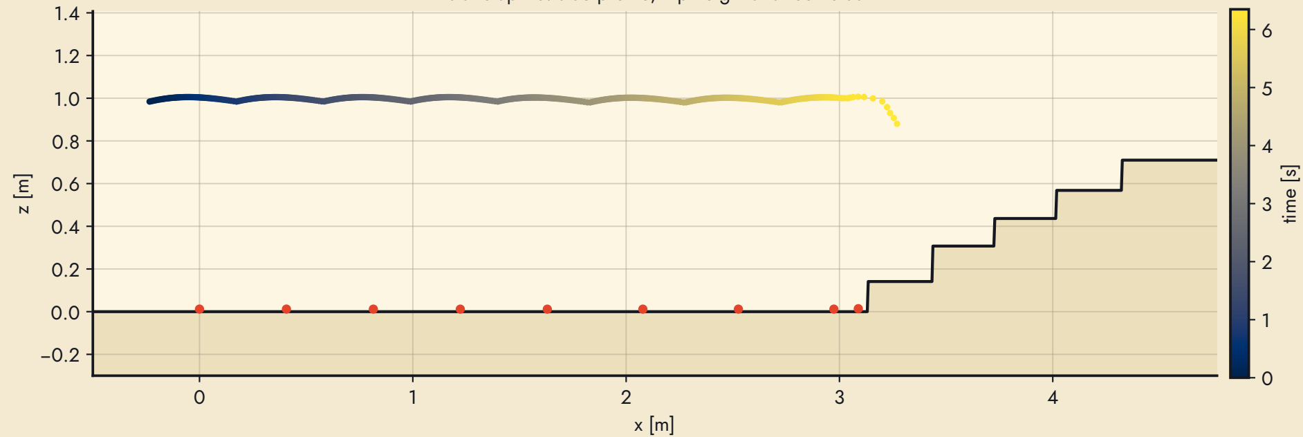
Stairs up #8: side profile, hip height and footholds
