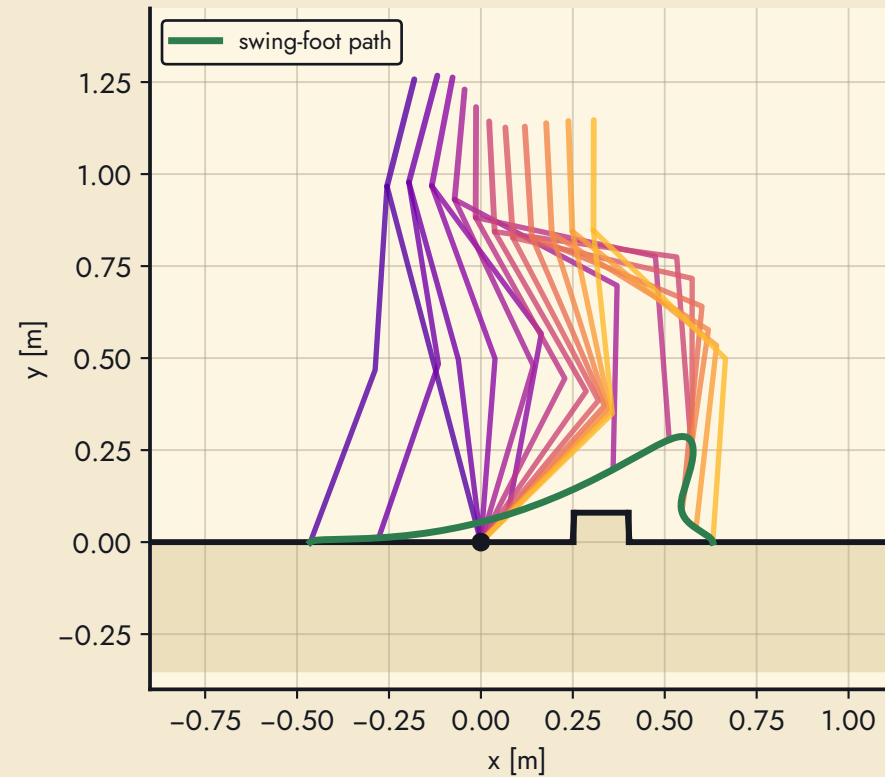
case 0: leading leg over the box (0.63 m step)
