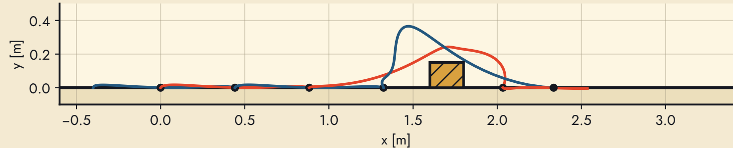
case 1: swing-foot paths of the whole plan (perceived box 1.59 m / 18 cm / 16 cm; true 1.60 / 20 / 15)
