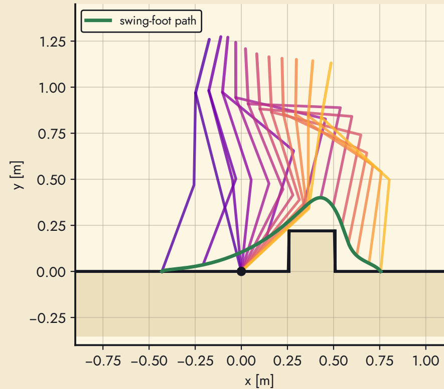
case 2: leading leg over the box (0.76 m step)
