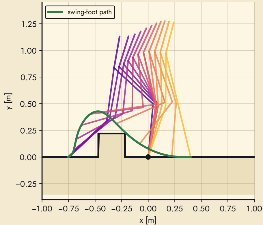
case 2: trailing leg over the box (0.40 m step), then the recovery step
