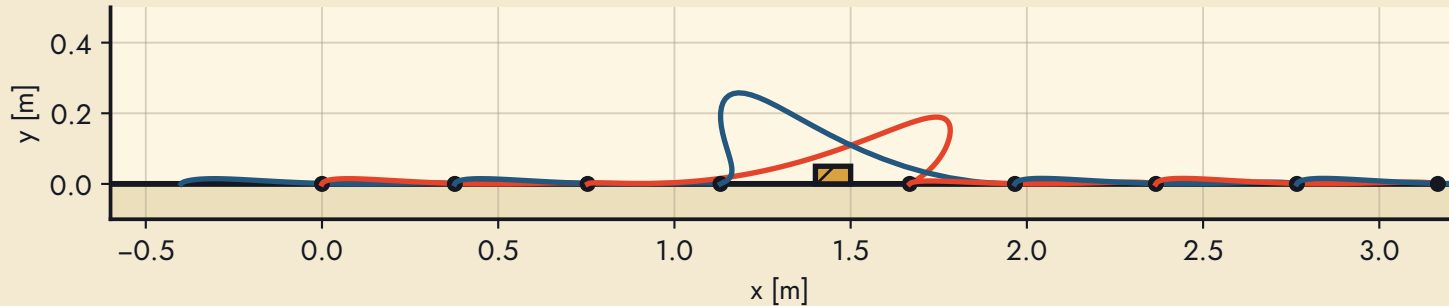
case 4: swing-foot paths of the whole plan (perceived box 1.40 m / 9 cm / 6 cm; true 1.40 / 10 / 5)
