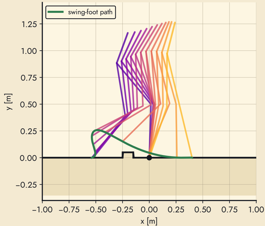
case 4: trailing leg over the box (0.40 m step), then the recovery step
