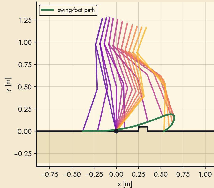
case 4: leading leg over the box (0.54 m step)
