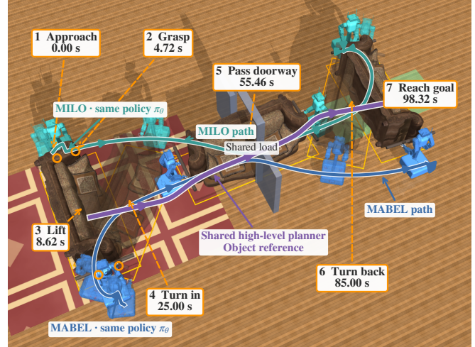
Fig. 1. Recorded cooperative transport (seed 142000). Both robots execute the same local policy with references from one shared high-level planner; a supervisor selects phase and height. Seven stages and timestamps show approach, grasp, lift and doorway reorientation. Blue/teal curves are measured MABEL/MILO base paths; purple is the planned object path. Curves are projected onto the floor and overlaid for visibility. Translucent poses expose intermediate motion; orange rings mark grasp locations and cutaway walls show the doorway.
