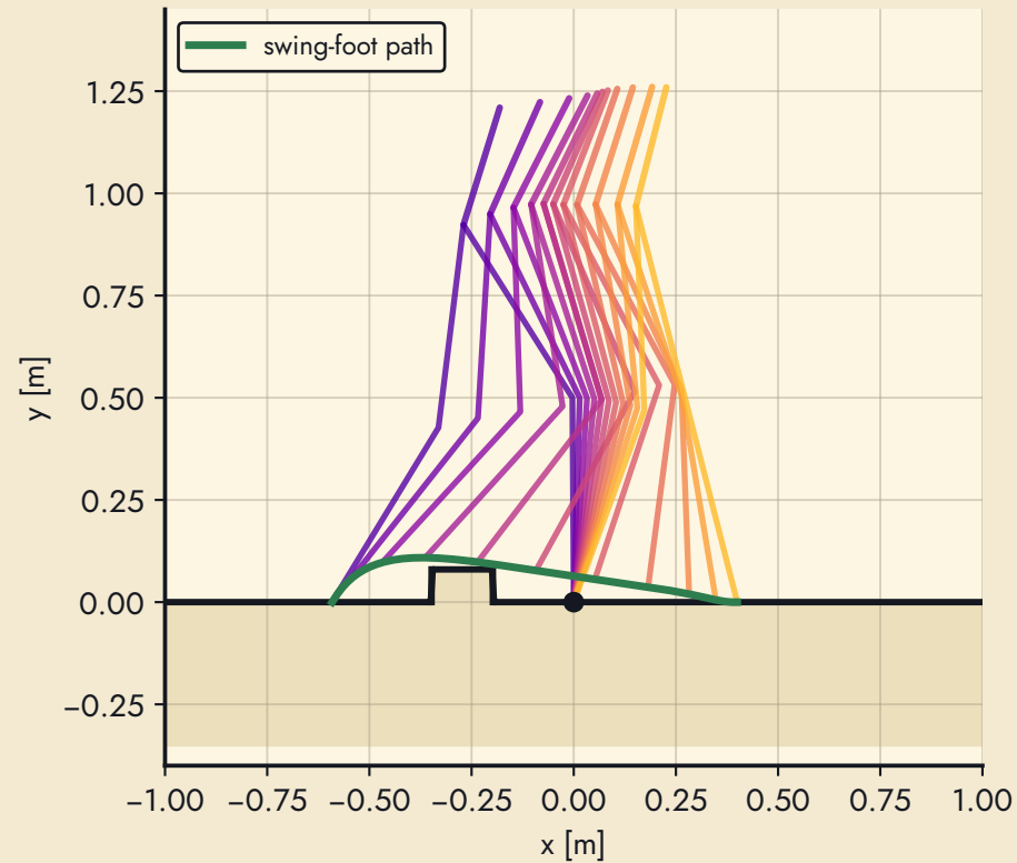
case 0: trailing leg over the box, back to the 0.40 m gait
