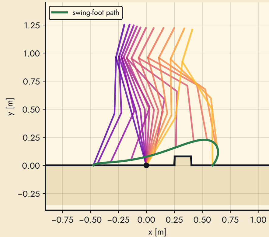
case 0: leading leg over the box (0.59 m step)
