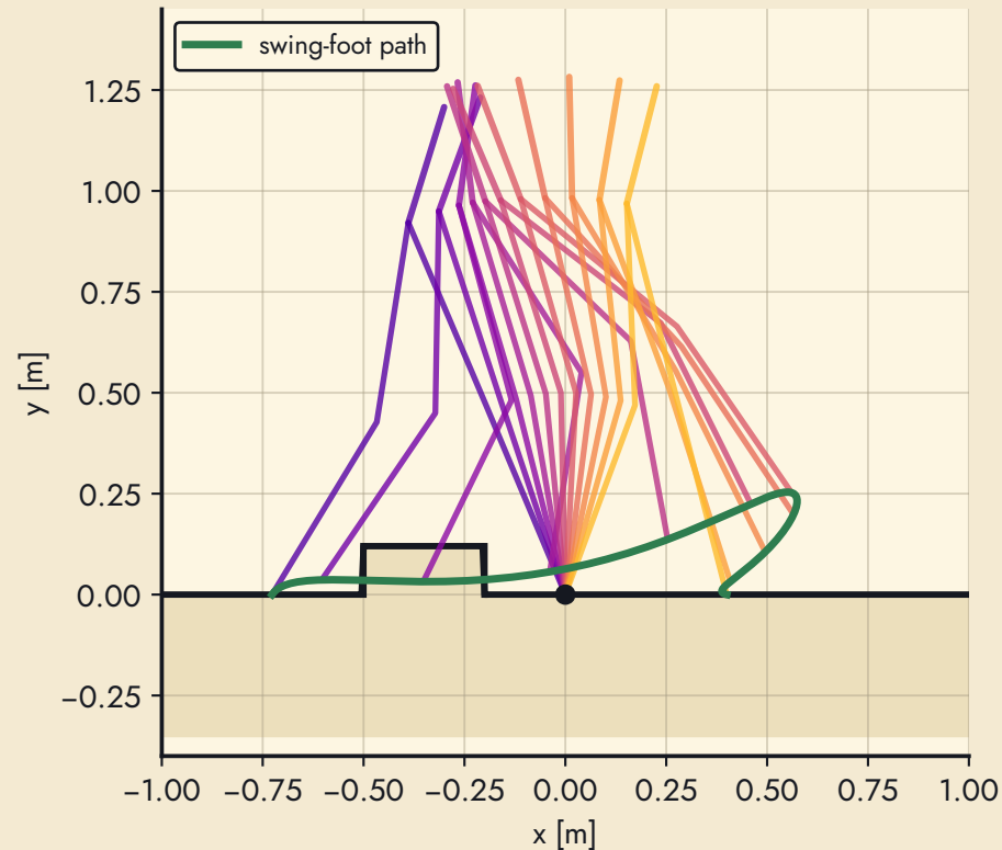
case 3: trailing leg over the box, back to the 0.40 m gait
