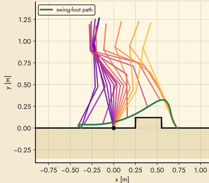
case 3: leading leg over the box (0.73 m step)
