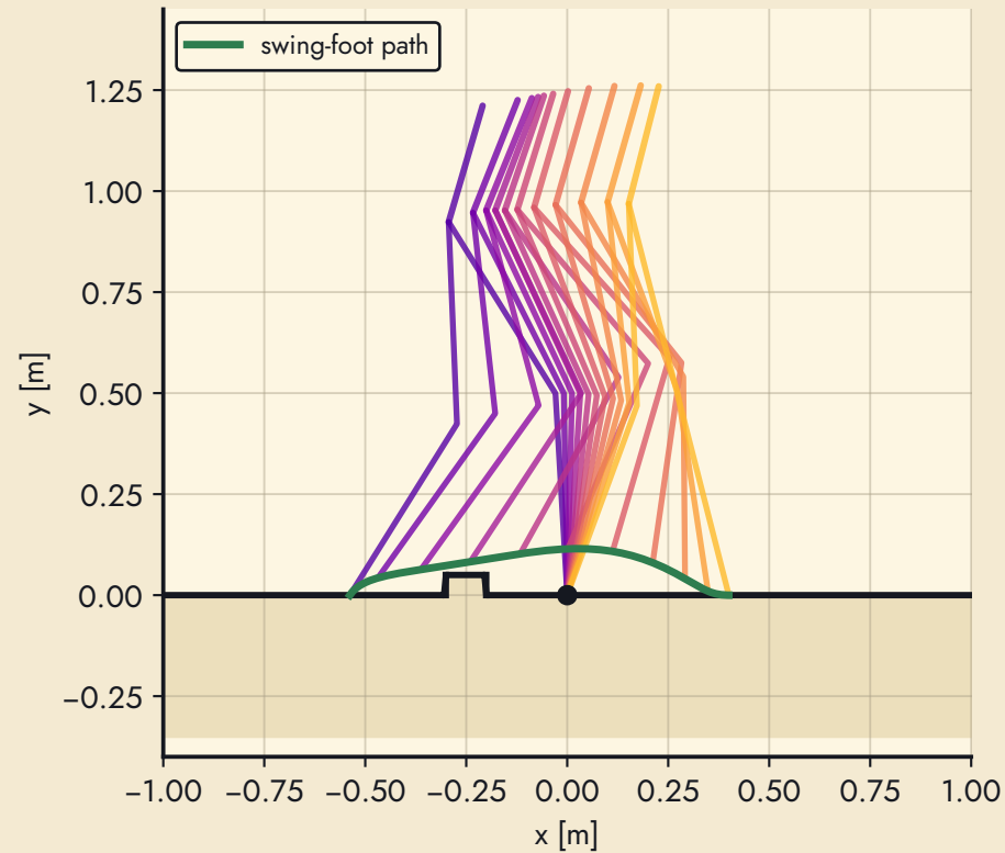
case 4: trailing leg over the box, back to the 0.40 m gait
