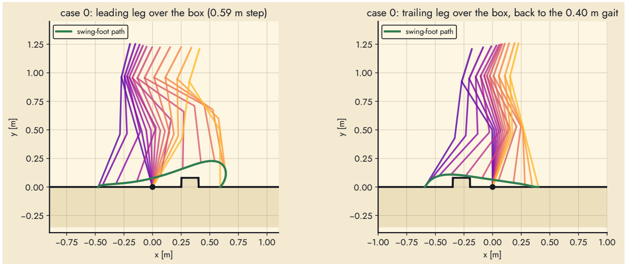
Figure 15: Case 0: the two chained step-over gaits over the perceived box (left: leading leg, right: trailing leg returning to the regular gait).
