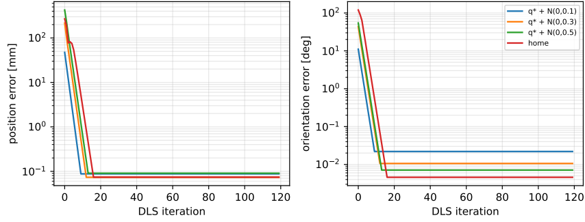
Figure 5: Damped-least-squares convergence to the palm-up target from seeds around the global solution and from the Panda home pose.
