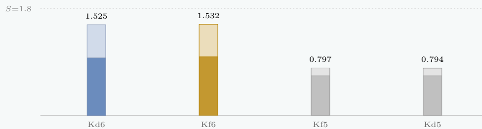
Figure 3.6: FIG-2.3: Iteration 3 (Selection recursed twice before expanding). Kf6 selected ( S = 1.53183 ). Selection does not stop at root; it recurses down Kf6 to expand leaf Kf8 (depth 2). Leaf value +0.95129 backs up.
