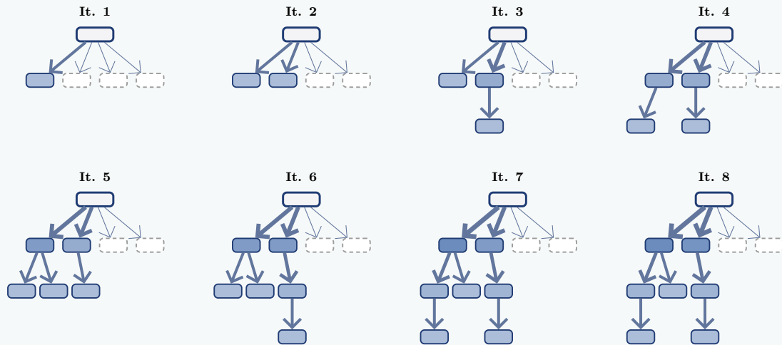
Figure 3.12: FIG-2.9: The whole search time-lapse. Sequence of tree states across iterations 1 to 8 showing structural growth.
