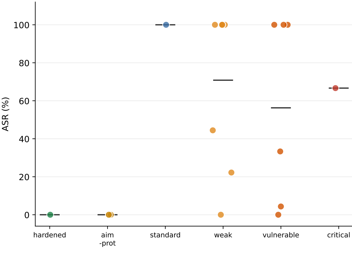
④ ASR vs ground-truth grade
