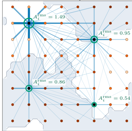
(c) rhizome: \mathbf{A}_i \kappa_{\theta} \mathbf{B}_j , update t=4
