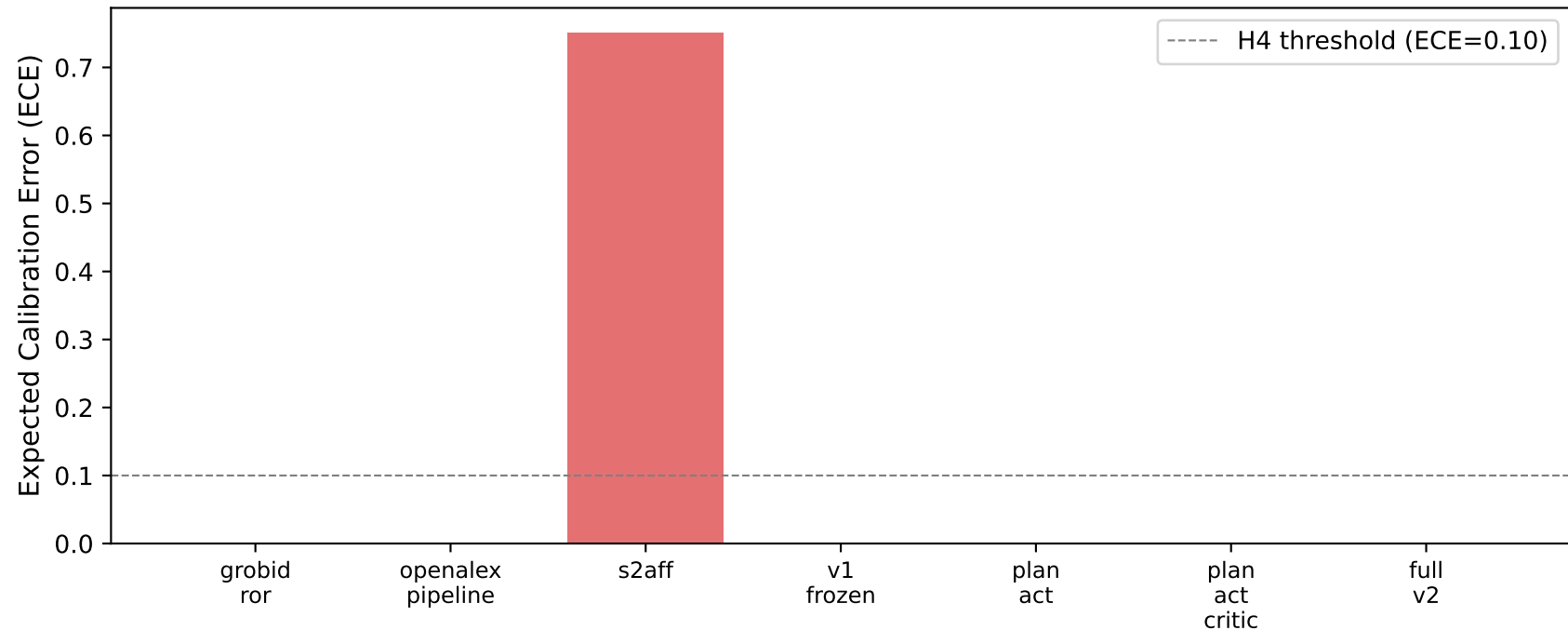
Figure 4.5 — Confidence calibration (ECE, lower is better)
