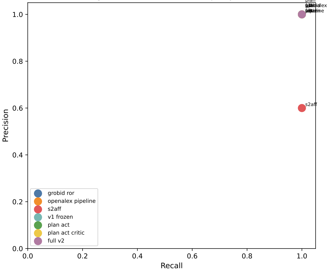
Figure 4.6 — Precision vs Recall per system
