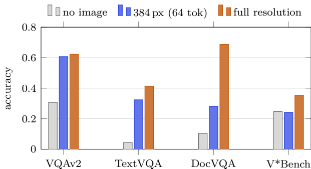
Figure 2: Accuracy per dataset at three information levels, 1000-example pilot. The gap between the blue and orange bars is everything escalation can ever buy, and it ranges from 1.6 points on VQAv2 to 40.7 on DocVQA. On V*Bench the thumbnail matches the blind baseline: at 384 px its small objects are simply gone.
