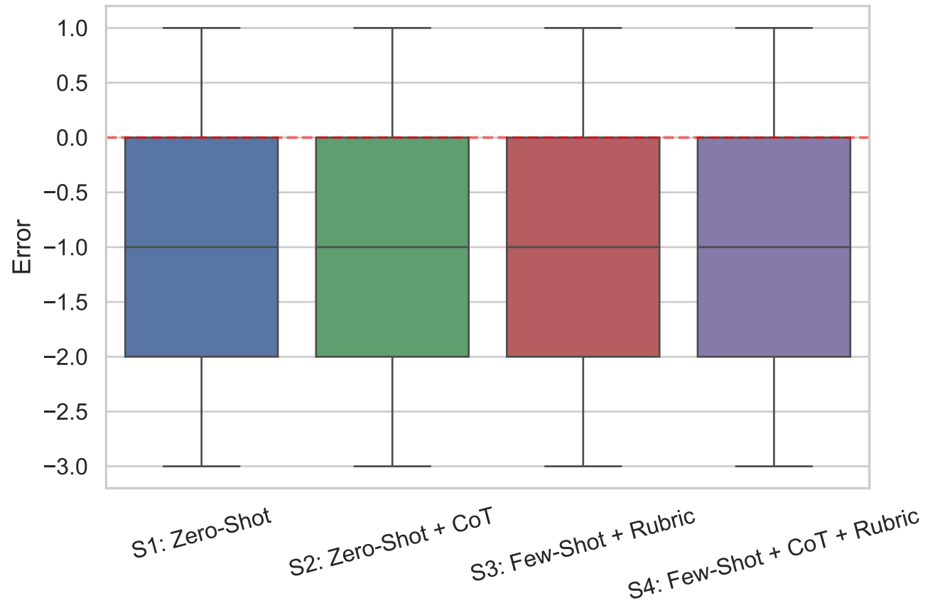
Score Error Distribution (Predicted – Human)
