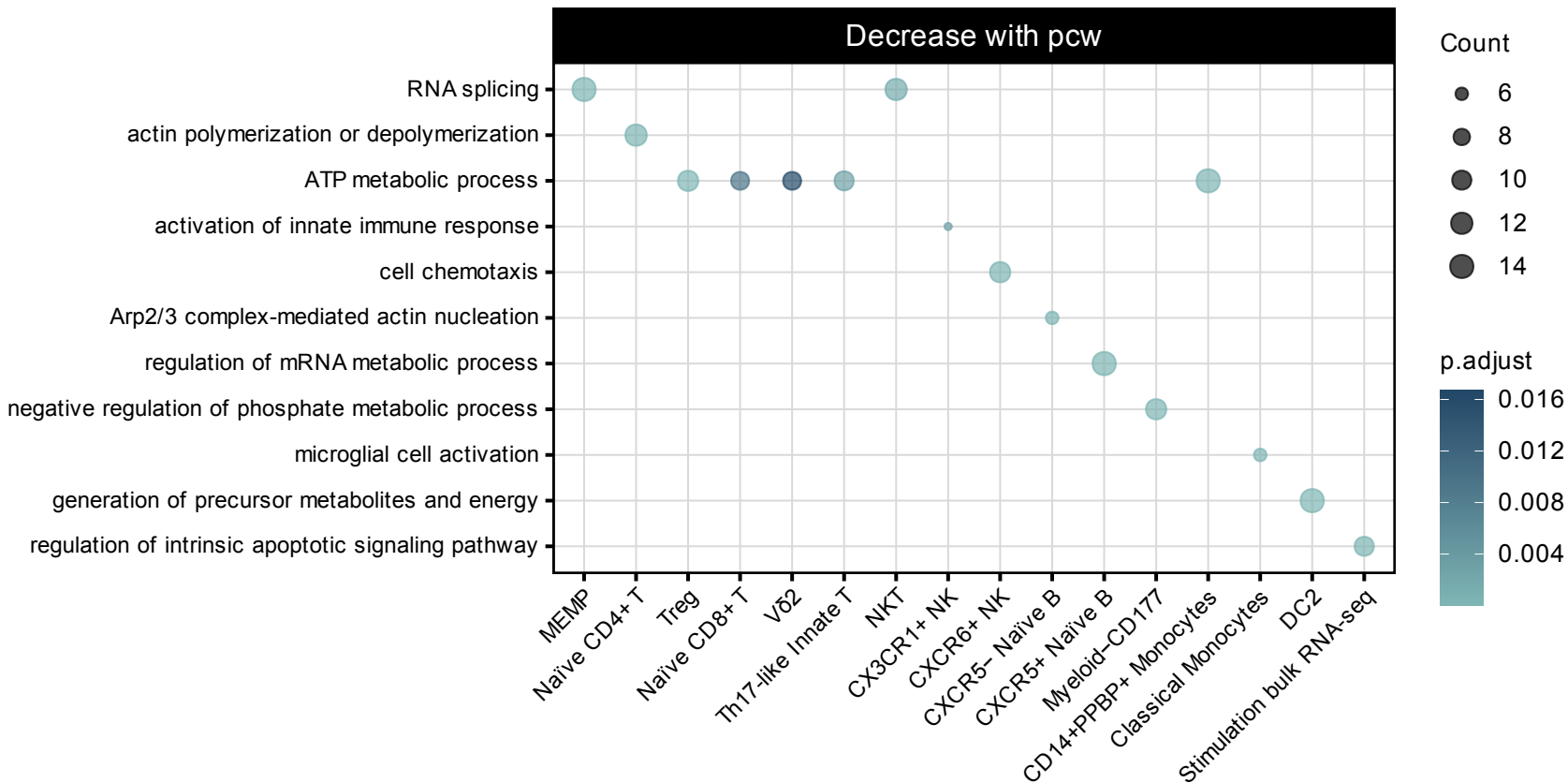
Top1 Pathways in Top100 Negative Features in Each View
