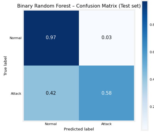
FIGURE 3.2: Normalized confusion matrix for binary Random Forest
