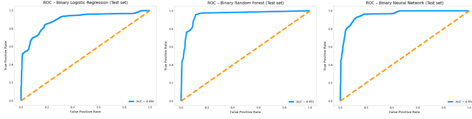
FIGURE 3.4: ROC curves for binary intrusion detection on test set
