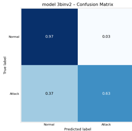
FIGURE 3.3: Normalized confusion matrix for binary Neural Network
