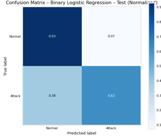
FIGURE 3.1: Normalized confusion matrix for binary Logistic Regression
