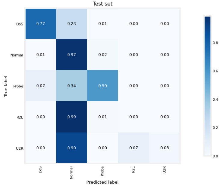
FIGURE 3.6: Confusion matrix for multi-class Random Forest on the test set
