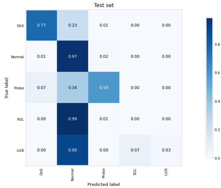
FIGURE 3.7: Confusion matrix for multi-class Neural Network on the test set
