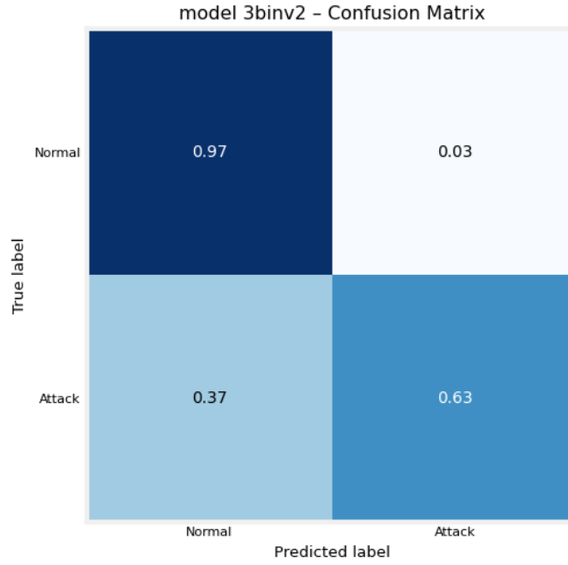
FIGURE 3.3: Normalized confusion matrix for binary Neural Network
