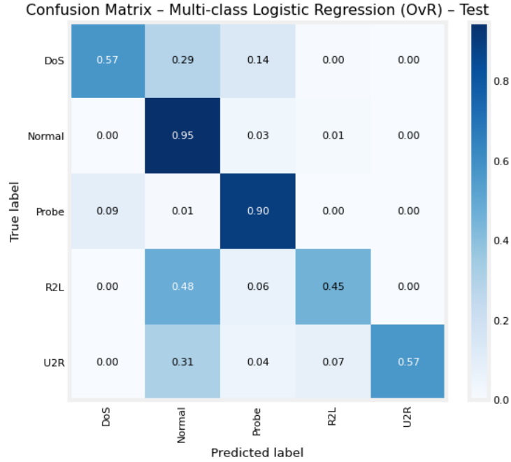
FIGURE 3.5: Confusion matrix for multi-class Logistic Regression on the test set
