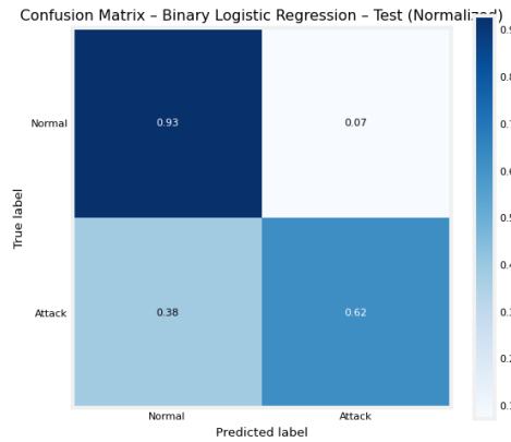
FIGURE 3.1: Normalized confusion matrix for binary Logistic Regression
