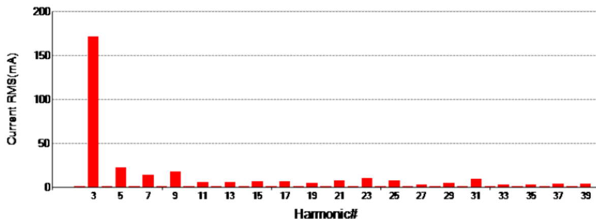
Harmonics Histogram
