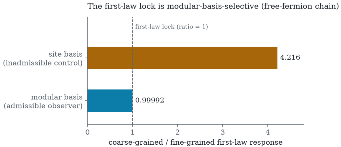
Figure 3: The selection mechanism on the lattice (q10_lattice_check.py; finite-size scan in fss_q10.py). Coarse-graining in the modular basis preserves the entanglement first law (ratio 0.99992; worst deviation 9.8 \times 10^{-7} across 36 configurations to L = 400 ); the site-basis control breaks it — the lock holds exactly for the coarse-grainings the Takesaki argument admits.
