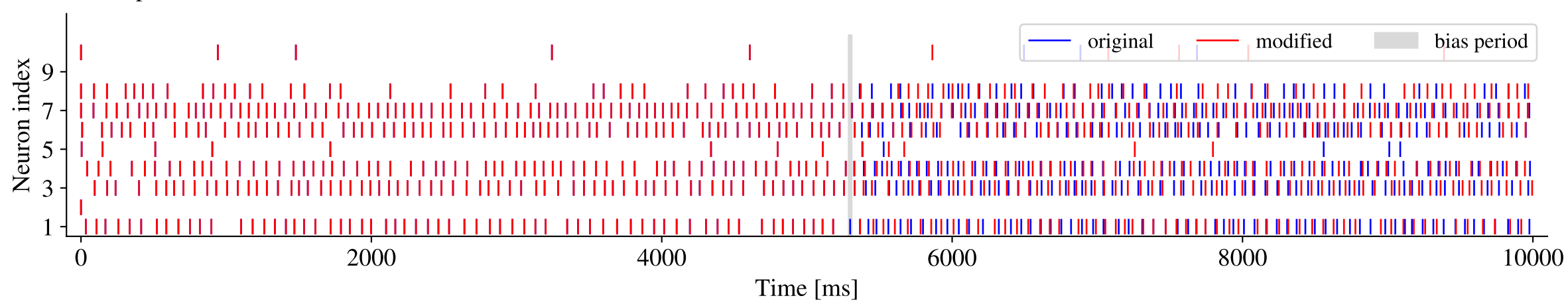
c Raster plot of the first 10 neurons
