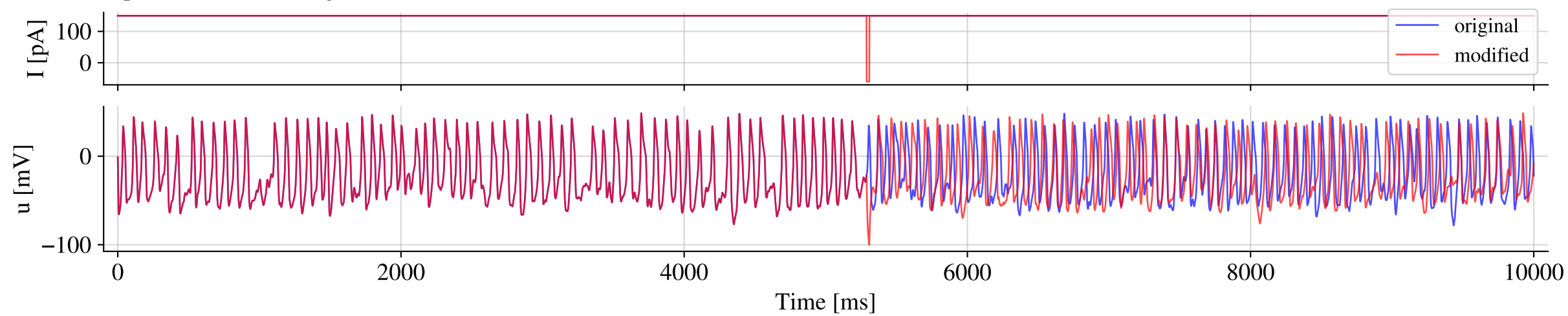
a Input current and voltage trace for neuron 1
