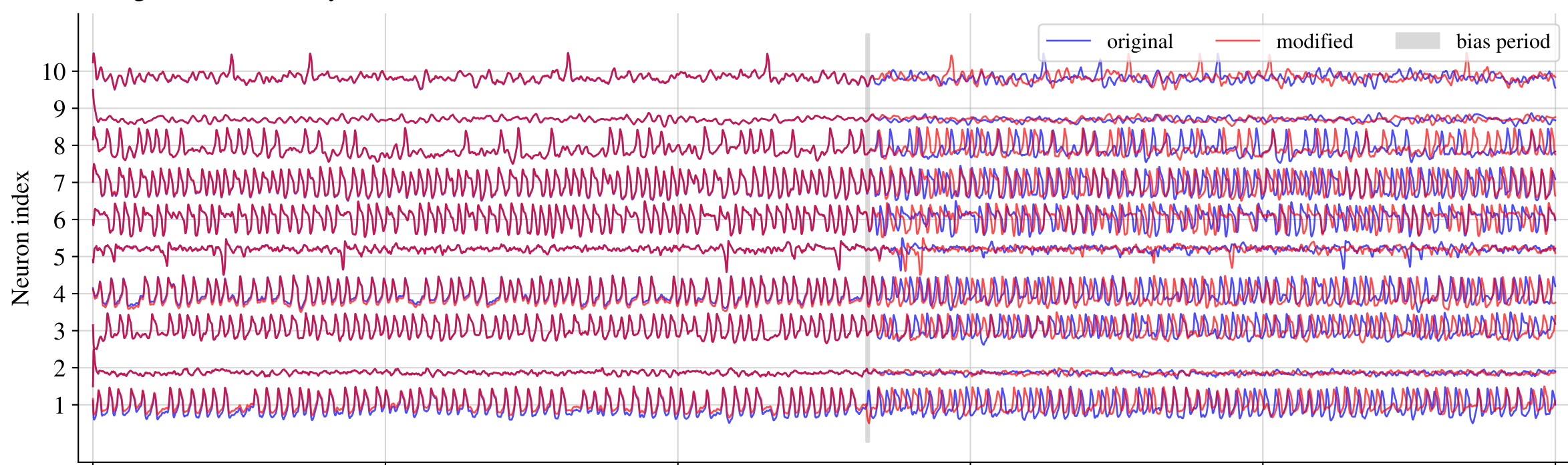
b Voltage trace of randomly selected neurons
