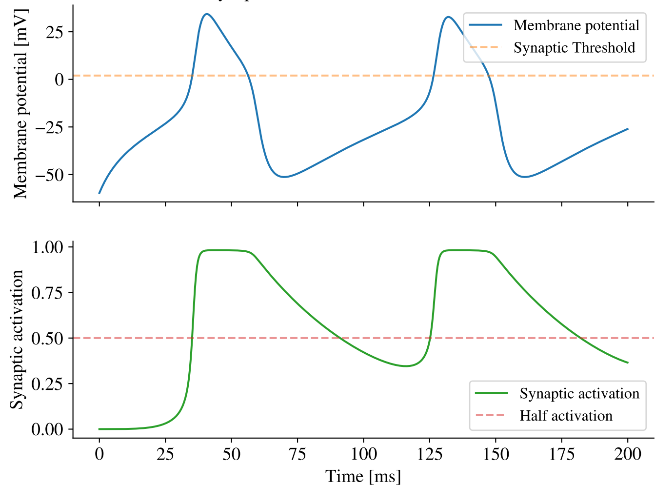
Synaptic activation in Morris-Lecar model
