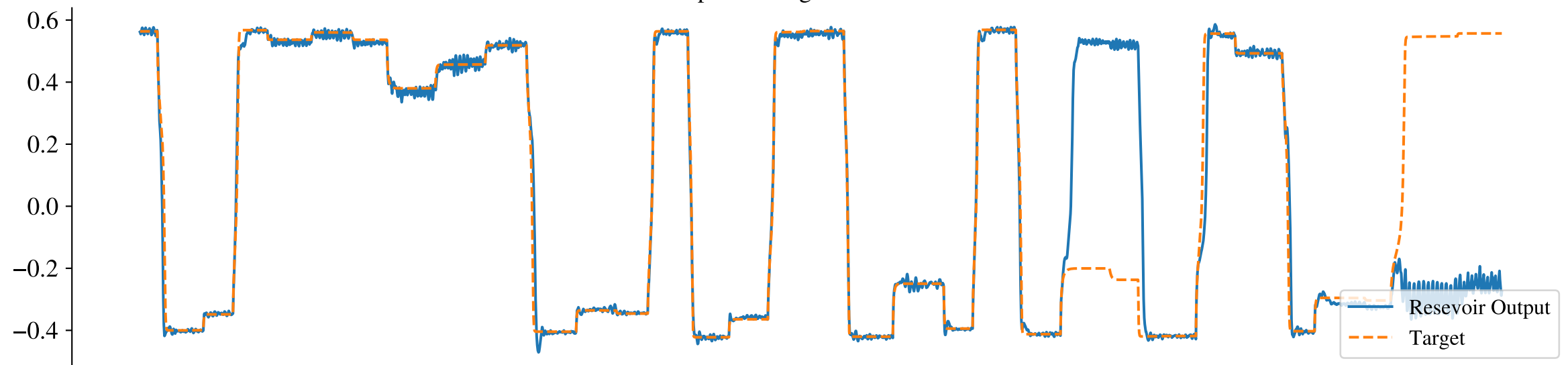
Reservoir Output vs Target for Pitchfork Bifurcation
