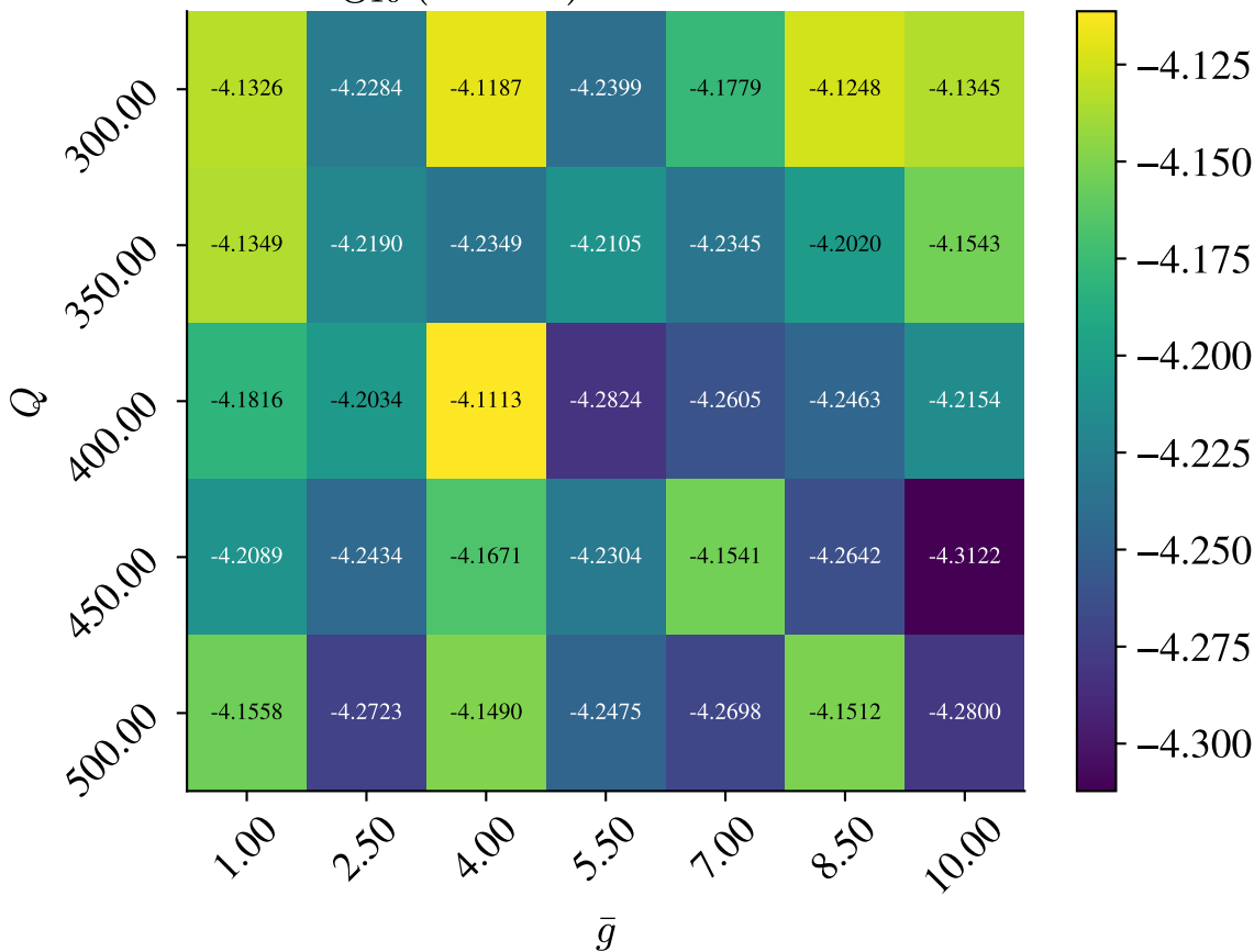
\log_{10} (RMSE) Evolution-based
