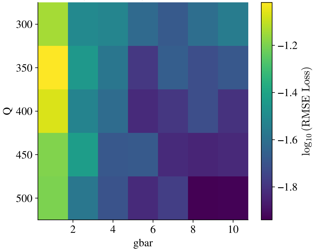
\log_{10} (RMSE Loss) for Current Model
