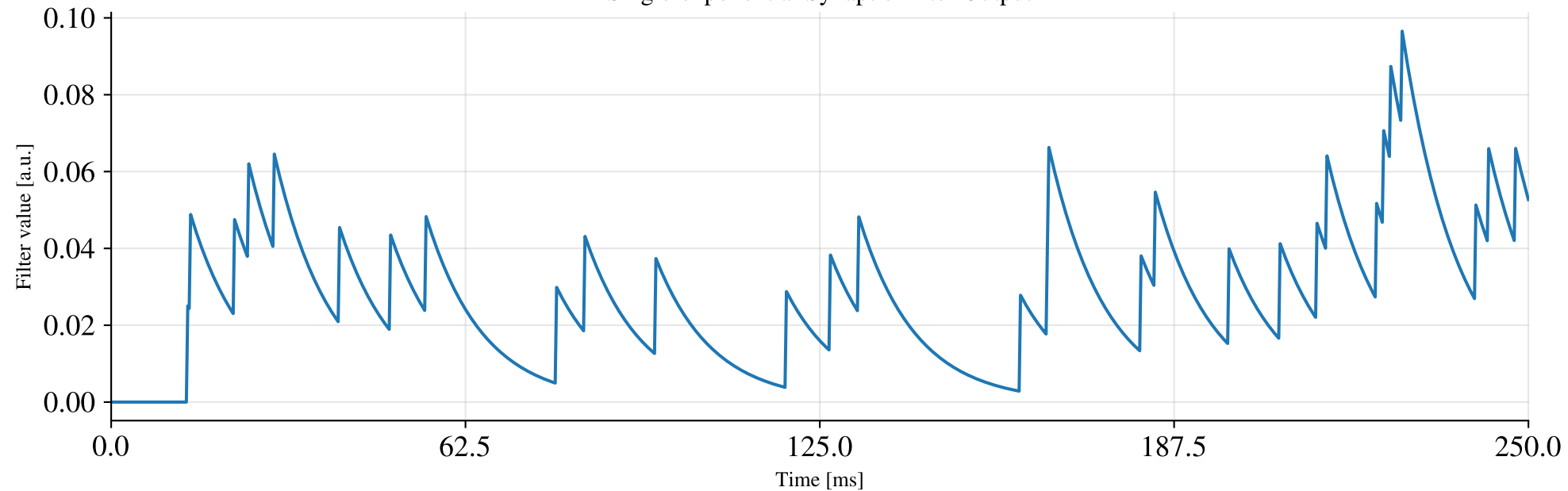
Single-exponential Synaptic Filter Output
