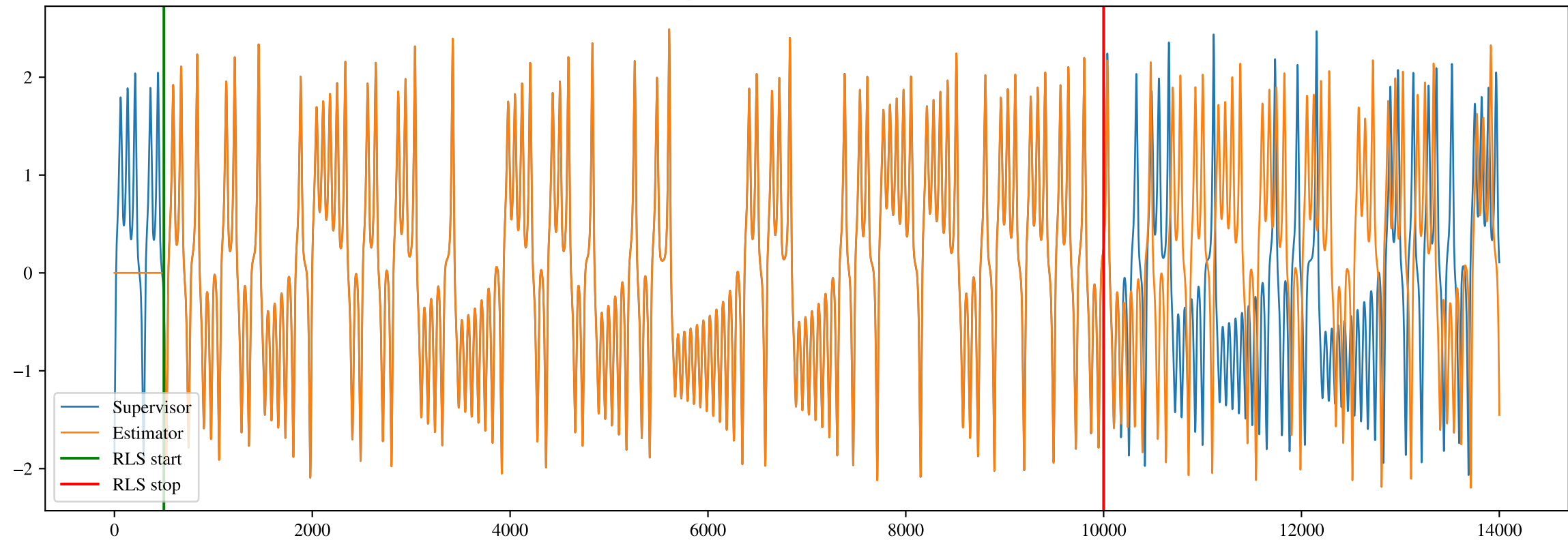
Model prediction for the Lorenz Attractor
