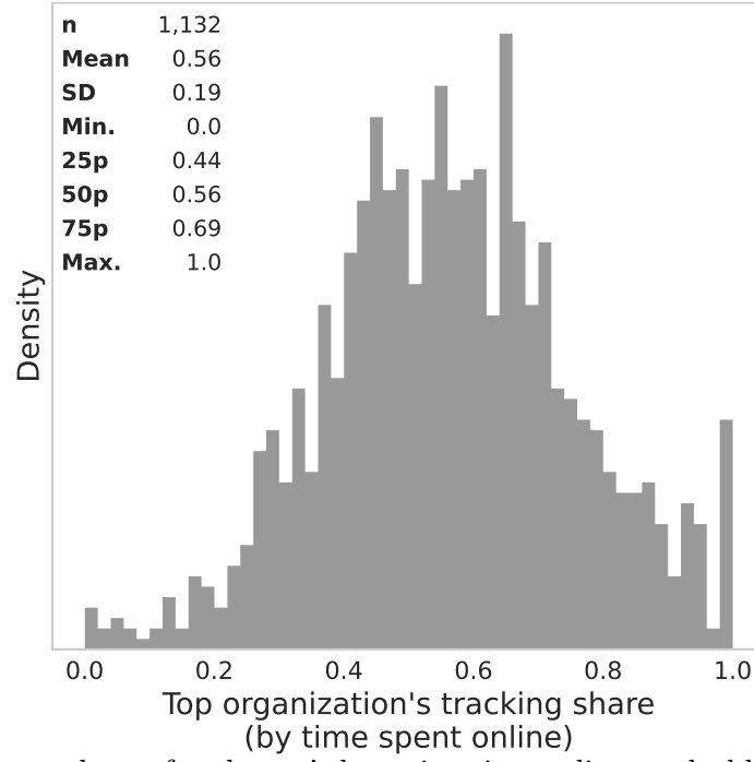
Figure E.1. The largest share of each user's browsing time online tracked by a single organization (Equation (5)):
