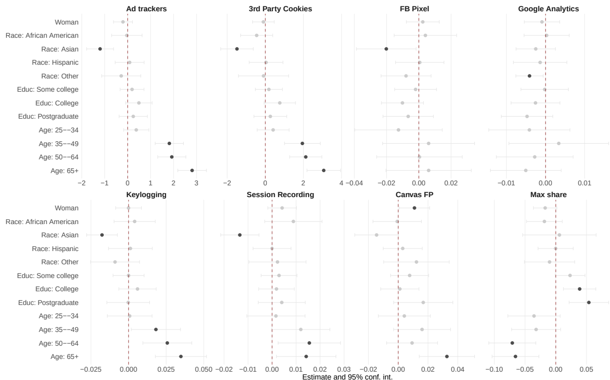
Figure 3. Demographic differences in exposure rate . Each panel reports OLS estimates and 95% confidence intervals from Equation (6) for the per-visit rate of each tracking method, and for the share of visits observed by the top organization. Black markers are significant at p < .05 . Full tables in Section D.
