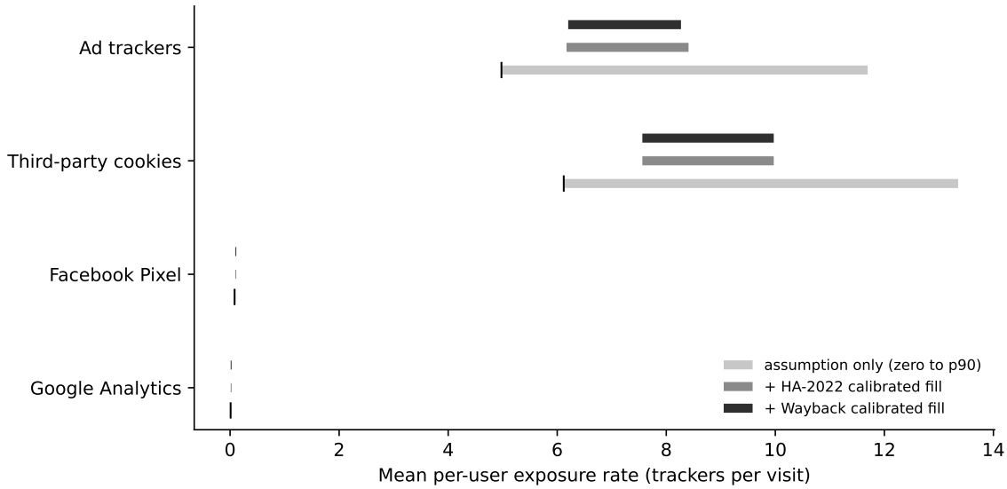
Figure C.3. Bounds on mean exposure rates under assumption-only and measurement-calibrated fills for unscanned visits.
