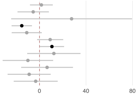
Session Recording
