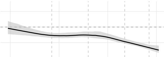
Session Recording
