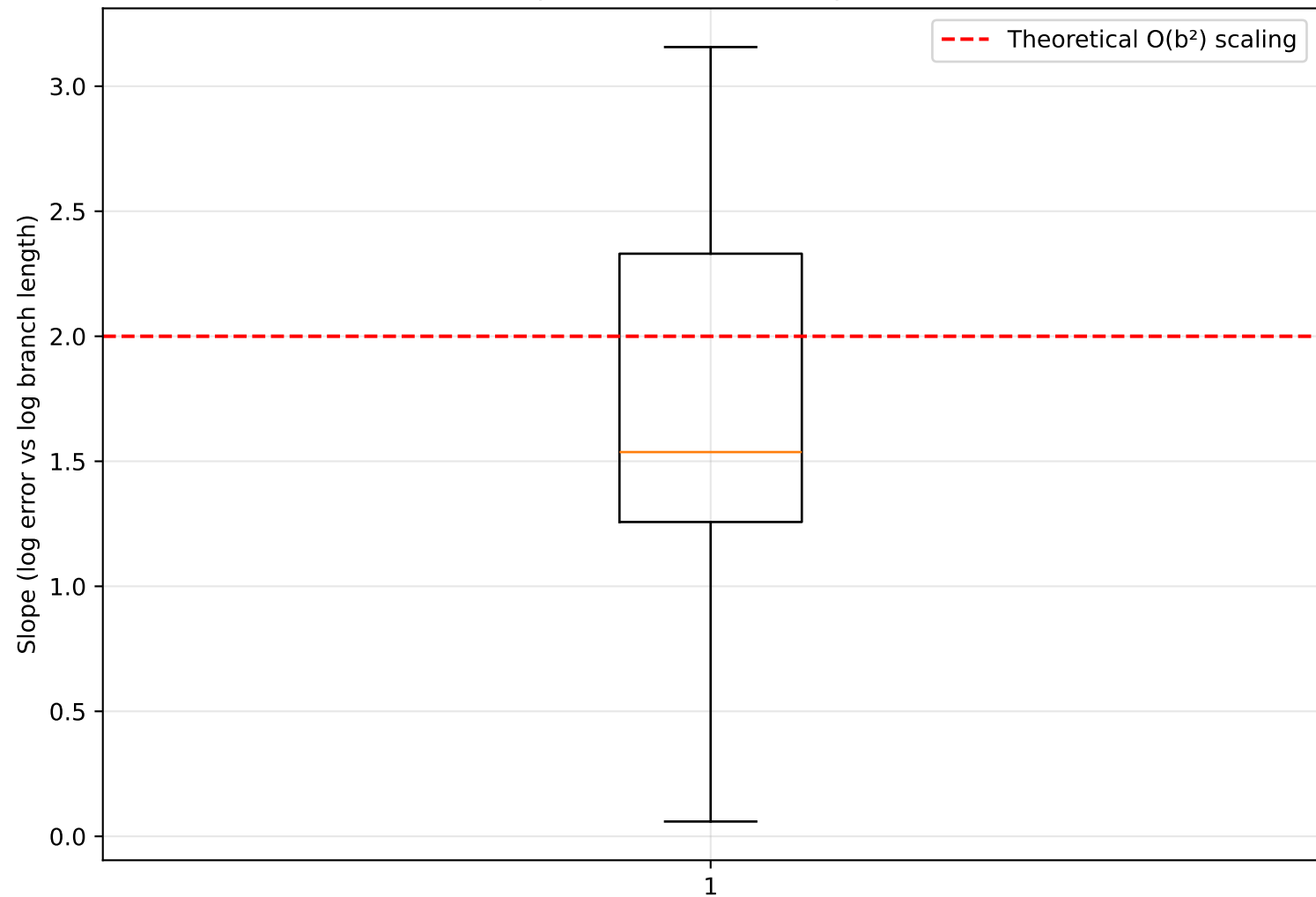
Error Scaling Slopes (Epistasis=0.5, n=100 pairs)
