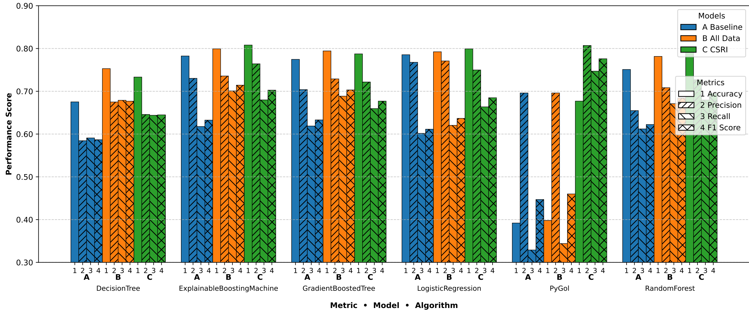
Model & Algorithm Performance Comparison
