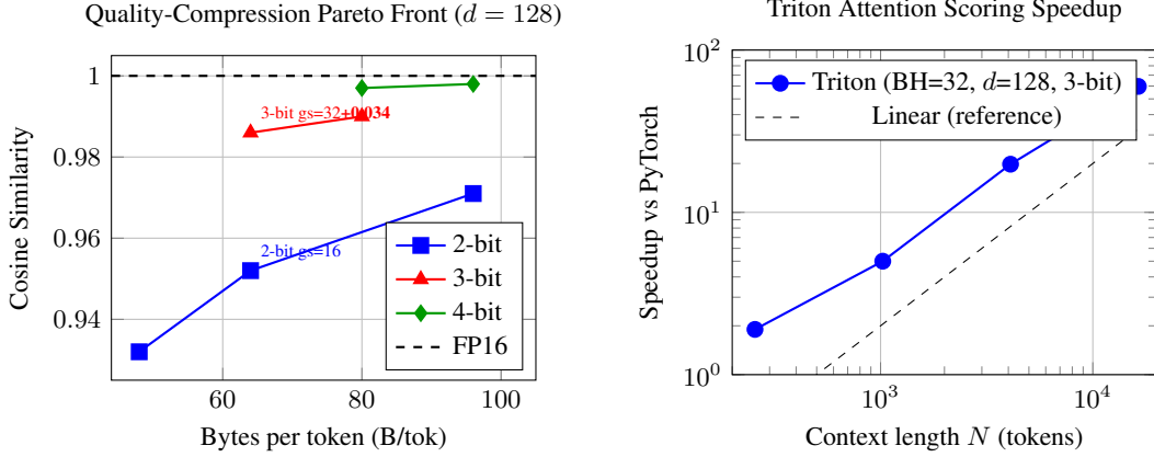
Figure 1: Left: Quality-compression Pareto front. At 64 B/token, 3-bit gs=32 (red, \text{CosSim}=0.986 ) is +0.034 above 2-bit gs=16 (blue, \text{CosSim}=0.952 ) at equal storage. The old default (2-bit gs=32 , 48 B/tok) is Pareto-dominated by 3-bit. Right: Triton attention scoring speedup vs PyTorch at increasing context length. Triton approaches constant-time behavior (sub-linear scaling) due to compressed key reads; 60\times speedup at N = 16,384 .
