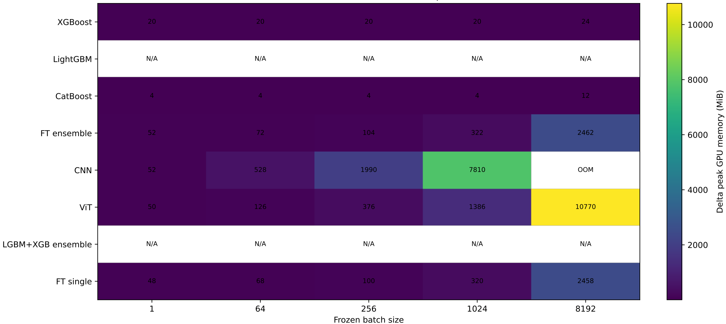
Single-T4 delta peak process GPU memory (MiB) Non-PASS outcomes retained; no imputation
